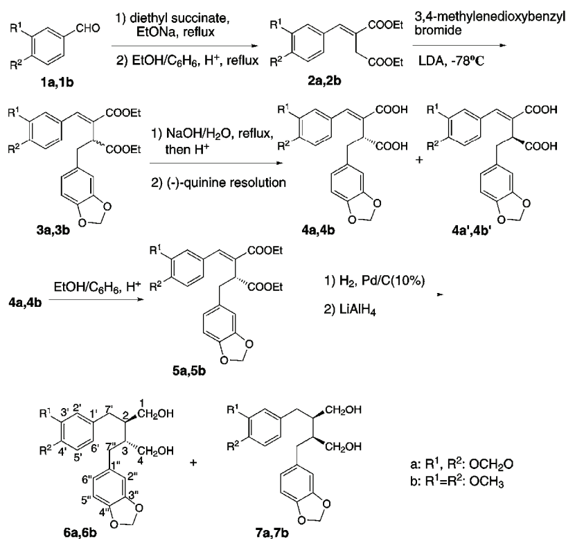
Scheme 1. Synthesis route of the compounds 2–7. The starting materials were piperonal ( 1a ) and veratraldehyde ( 1b ). Condensation of 1a or 1b with diethyl succinate in EtONa/EtOH solution afforded the benzylidene half-ester, which was followed by esterification to produce the diester 2a or 2b . Treatment of 2a or 2b in THF with LDA and 3,4-methylenedioxybenzyl bromide at –78 °C afforded the diester 3a or 3b . Then compound 3a or 3b was hydrolyzed to form the diacid. At this stage, the diacids were resolved via the quinine salt. The quinine salt of diacid (–)- 4a or (–)- 4b crystallized first. Concentration of the mother liquors gave a solid, which yielded the quinine salt of (+)- 4a' or (+)- 4b' . The diacid 4a or 4b was esterified to produce diester (–)- 5a or (–)- 5b . The diester 5a or 5b was hydrogenated under an H 2 atmosphere, followed by reduction with LiAlH 4 in THF to produce a readily separable mixture (approximately 1:1) of diols threo -(–)- 6a and erythro - 7a or threo -(–)- 6b and erythro -(–)- 7b .
