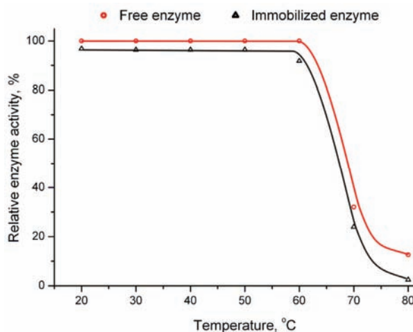
Fig. 5. Temperature stability of \beta -glucosidase covalently bonded onto mesoporous silica support (pore size 29 \text{ nm} ).
