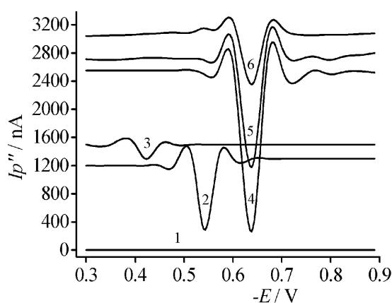
Fig. 1. Second order derivative linear sweep voltammograms of the Cup–Pb(II)–CS interaction system. 1. pH 5.5, HAc–hexamine; 2. 1 + 5.0 \times 10^{-5} \text{ mol L}^{-1} Cup; 3. 1 + 2.5 \times 10^{-5} \text{ mol L}^{-1} Pb(II); 4. 1 + 5.0 \times 10^{-5} \text{ mol L}^{-1} Cup + 2.5 \times 10^{-5} \text{ mol L}^{-1} Pb(II); 5. 4 + 10.0 \text{ mg L}^{-1} CS; 6. 4 + 20.0 \text{ mg L}^{-1} CS. The potentials are expressed vs. SCE.
