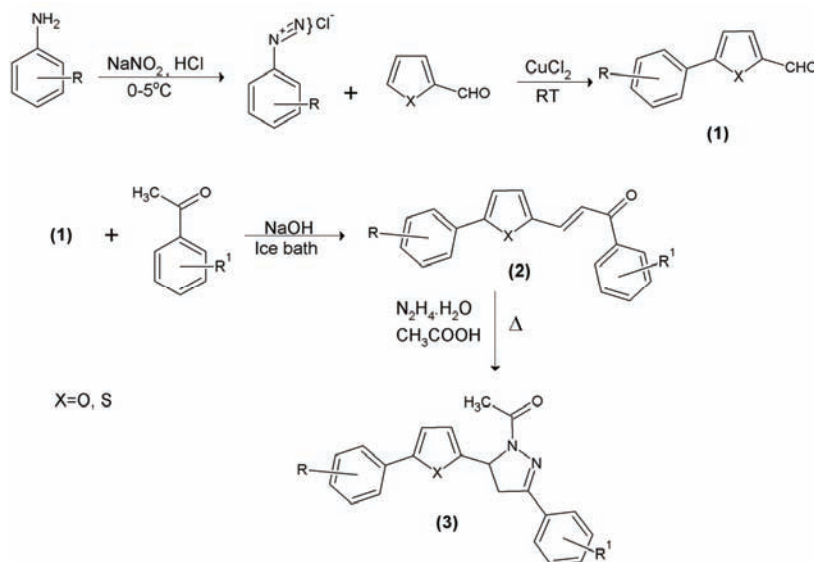
Scheme 1. The schematic route for the synthesis of the N -acetyl-3-aryl-5-(substituted aryl-2-furyl/thienyl) pyrazolines.
